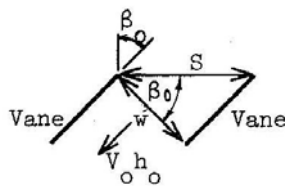
(a) Vane channel width and vane angle
