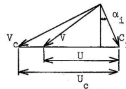
(b) Critical vane speed
